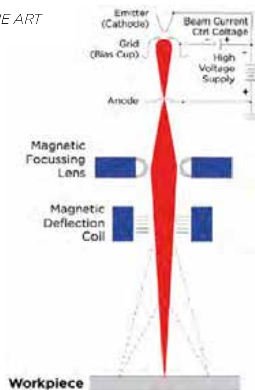
Fig. 4.1: The principle of electron-beam generation and direction for focused beam applications under vacuum conditions.
