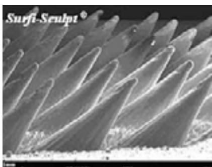
Fig. 4.10: e-beam surface-structuring by Surfi-Sculpt®, developed by The Welding Institute (TWI), UK.
