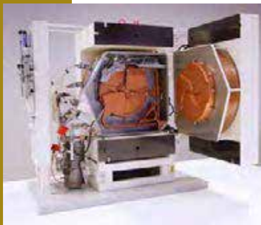
Fig. 3.15: (Left) a 16-MeV radionuclide production cyclotron from GE; (right) an 11-MeV radionuclide production cyclotron from Siemens, including the system for the production of the radiopharmaceuticals.
